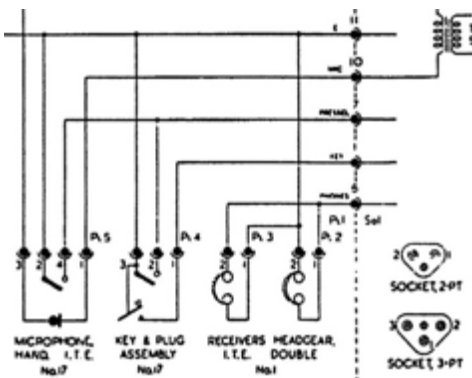
Part of circuit diagram showing connections of Key and Plug Assembly No. 17 to the No. 42 Set.
