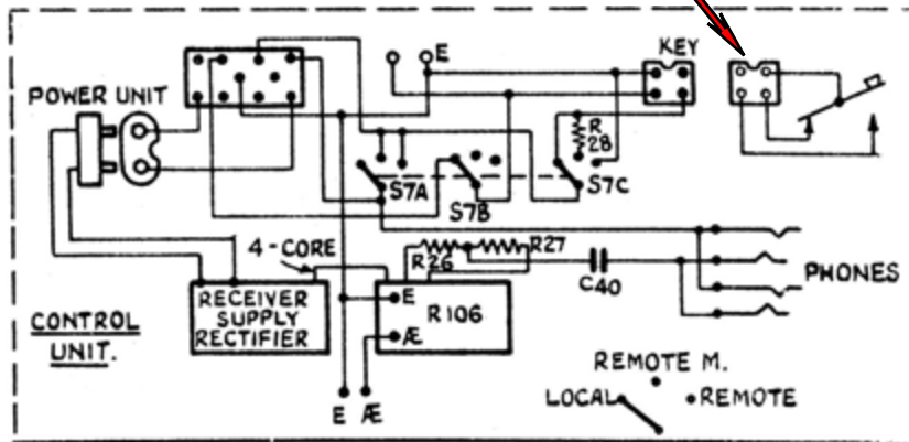
Part circuit diagram of Wireless Set Special type 6X1 showing connections to Morse key. Note that the break (space) contact was used, hence the use of a 4-point plug and socket.
