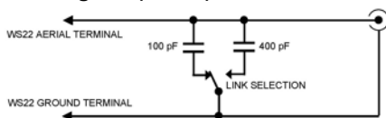
Aerial Coupling Equipment, Set Unit JT (above) and circuit diagram (below).
