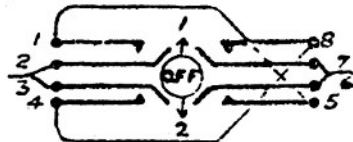
POTENTIOMETER SWITCH
