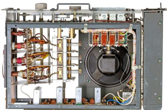
Bottom view of the FRM-2 receiver showing battery compartment (separate unit right), control push buttons (top right), IF pcb (bottom), AF pcb (right) and RF assembly (left).
