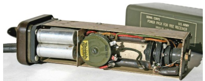
Chassis view of the opened power pack as seen from either side.
