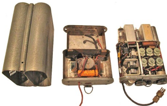
Combined battery box/receiver case, battery box with loudspeaker and receiver unit of Polish OP3-G.
