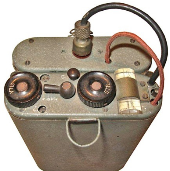
Top view of the OP3-G showing the receiver and battery box front panel. Note the metal ring used for removing the receiver chassis and battery box from the combined receiver/battery case. It replaced a leather strap used in earlier versions.
