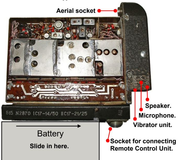
Internal view of the Alycha; note engraved serial number, organisation-group and channel numbers.
