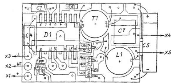
Top view of variation B board for 33012, intended for fitting in a terminal block.
