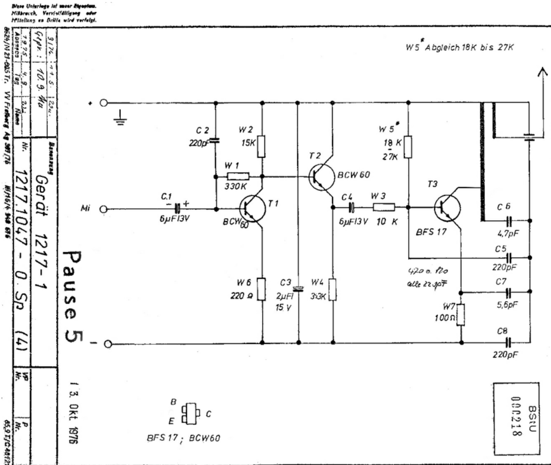
Circuit diagram of the original 31217-1 and 31217-11. The RF part differed very little from the earlier 31216-1. This early version was developed for an external magnetic microphone.
