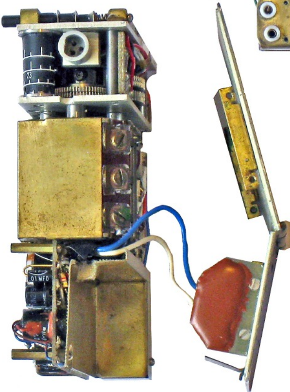
Right hand side view of RR-49 detached from the metal outer case. Note 3-point DC input and aerial socket.
