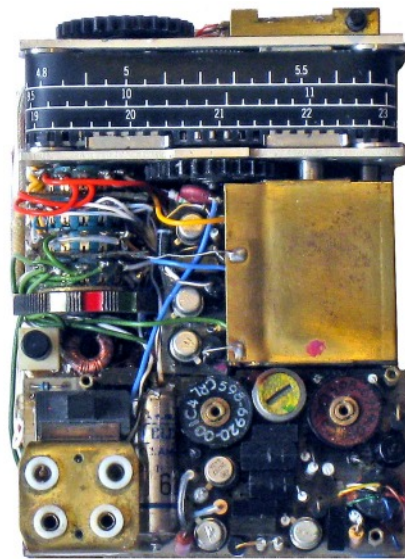
Top view of the RR-49 with its outer case detached (right). Note the metal tape frequency scale.
