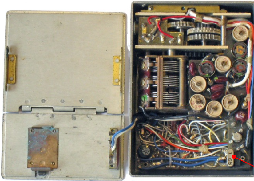
Internal view of RR-49 with bottom plate removed.
