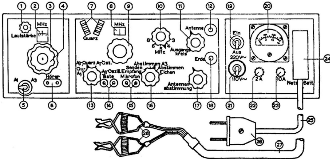
Drawing and two pages of the Yugoslav manual for the SEM-78. Note minor differences in construction compared to the set on the previous page. (Microphone socket, fuses and ground socket)
